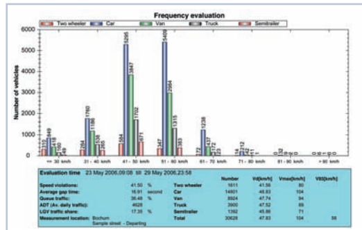
Some examples of data evaluation ( viasis speed information systems and viacount II traffic counter).
